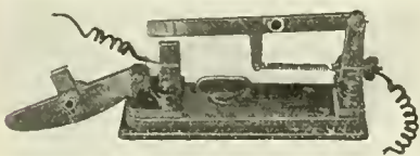
FIG. D. THE TRACK CIRCUIT BREAKER In falling position. Circuit broken.
